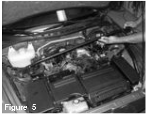
Figure 5 All four 12mm nuts have been removed and the strut tower bar is now pulled out.
