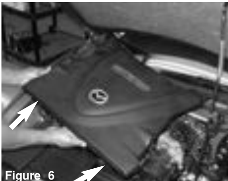
Figure 6 pull up on the stand offs located in front of the engine cover. A slight tug up will be required to pull the stand offs out of the stock grommet.
