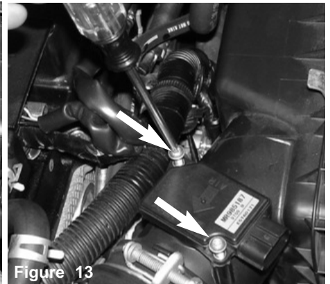
Figure 13 An allen screwdriver is used to loosen the two stock screws from the mass air flow sensor.
