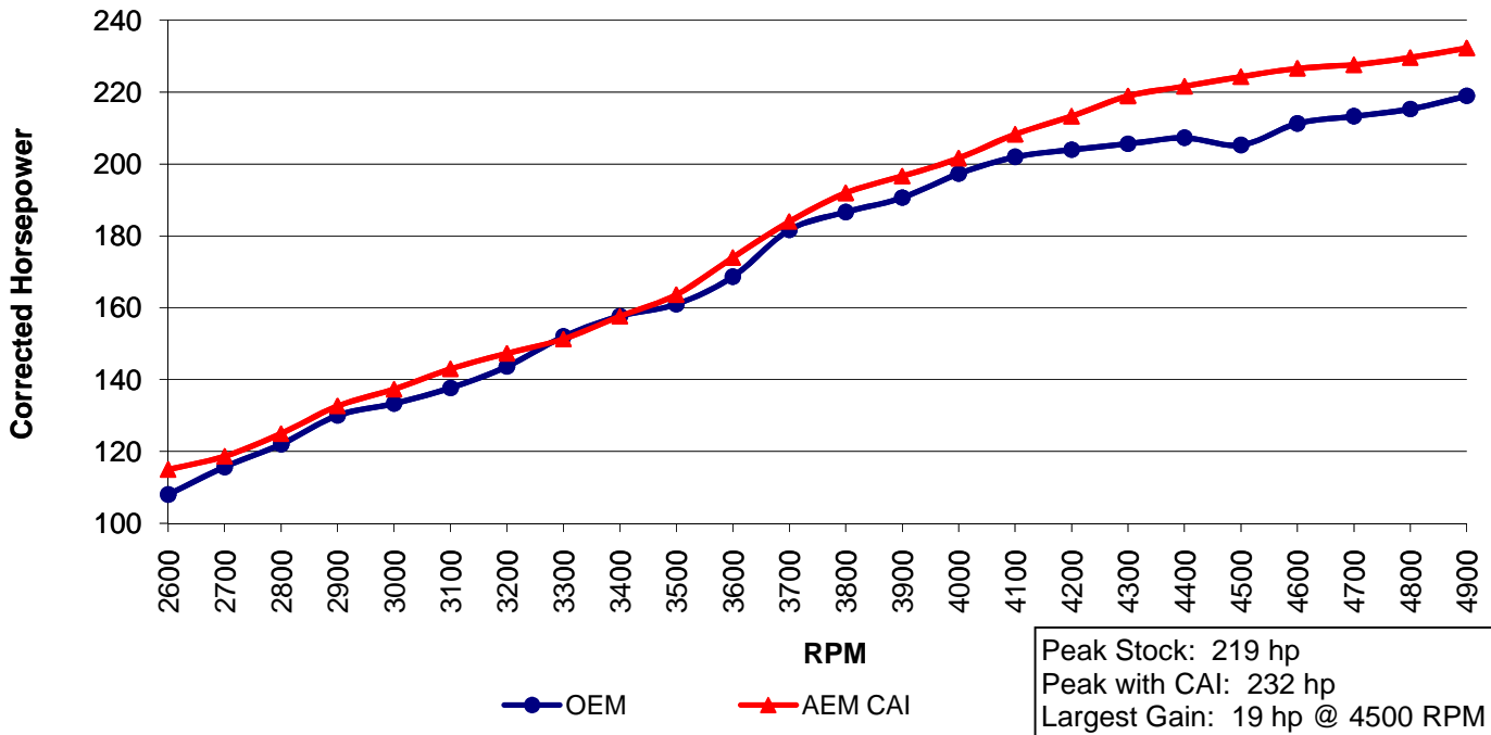
Corrected Horsepower (hp) vs. Engine Speed (RPM)
