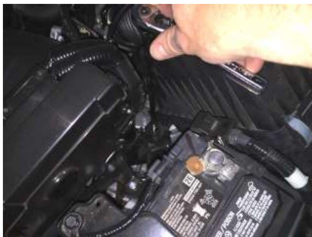
b. Remove the lower bolt securing the factory air box.
