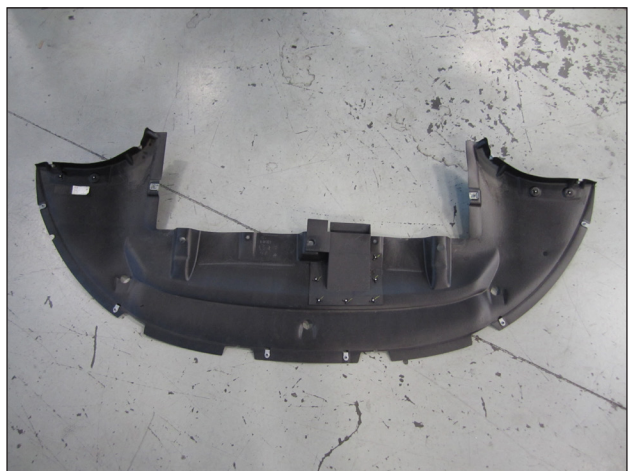
p. Remove the underside splash guard from between the front bumper cover and the belly pan.
