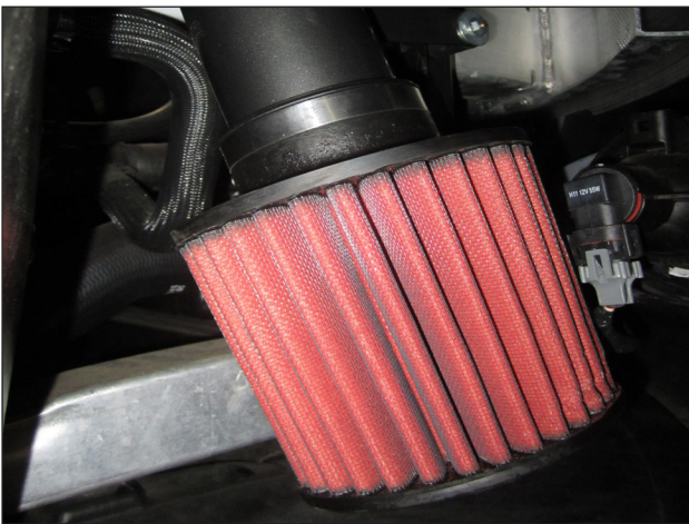
k. Install the #52 (F) hose clamp and the AEM Dryflow air filter (C) onto the lower intake tube. Fully tighten the hose clamp.
