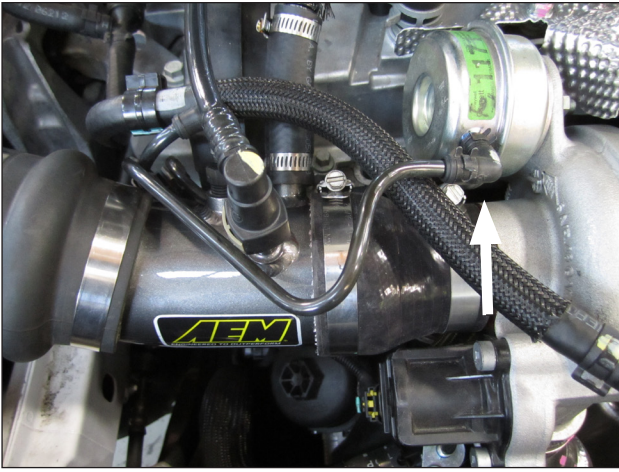
g. Re-connect the vacuum line elbow to the turbo wastegate actuator. Route the line as shown.
