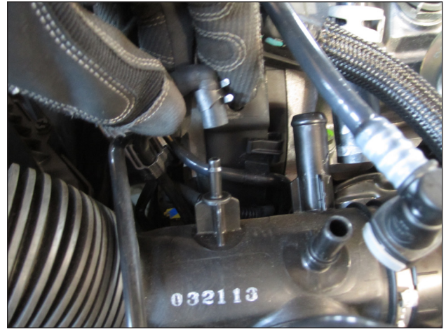
f. Disconnect the secondary vacuum line elbow from the intake tube.
