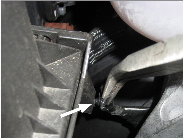
g. Remove the clip holding the wiring harness to the back of the air box with pliers.
