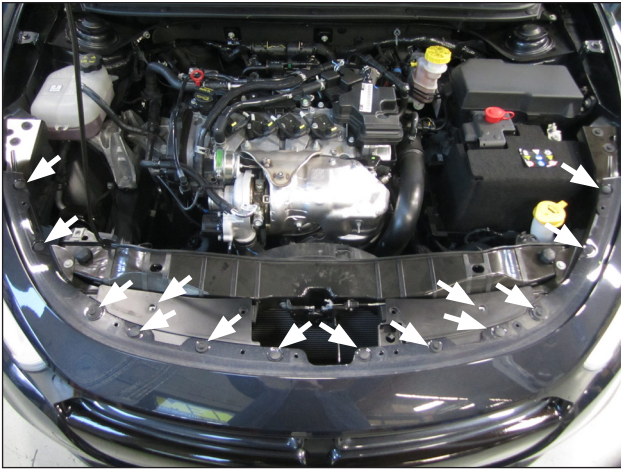
k. Next, remove the 8 clips and 6 bolts that hold the bumper cover onto the radiator core support.
