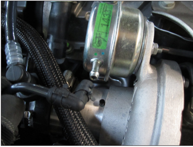
e. Disconnect the vacuum line elbow from the wastegate actuator at the turbocharger.
