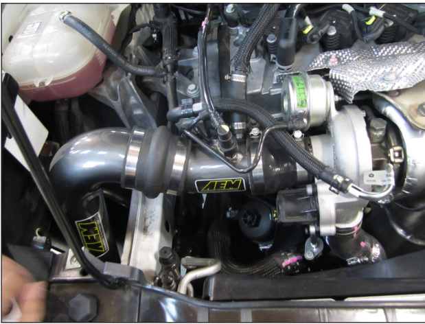
j. Install the lower intake tube (B) into the hump hose as shown. Do not tighten the hose clamp.
