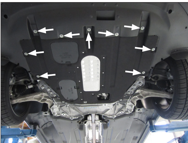
o. Remove the 9 M6 bolts around the front and side edges of the belly pan. Do not remove the belly pan.
