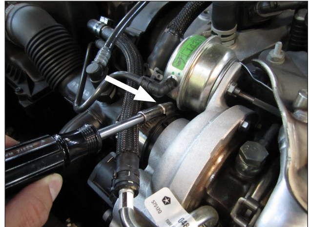
b. Loosen the hose clamp on the intake tube at the turbocharger inlet.
