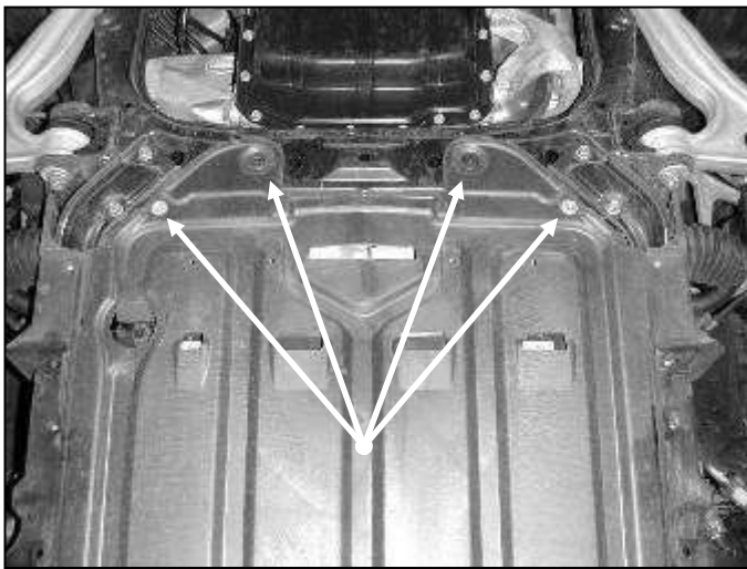
y. Loosen and remove the mounting bolts. Loosen and remove the push-in tabs. Remove the bottom fender liner.
