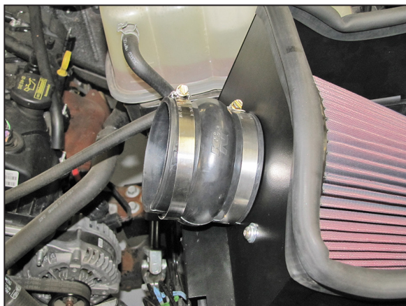
14. Install the provided hump hose (084057) onto the filter adapter and secure with the provided hose clamp.
