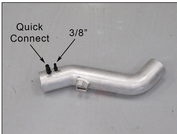
15. Install the Quick connect and 3/8" vent fitting into the K&N® intake tube as shown.
