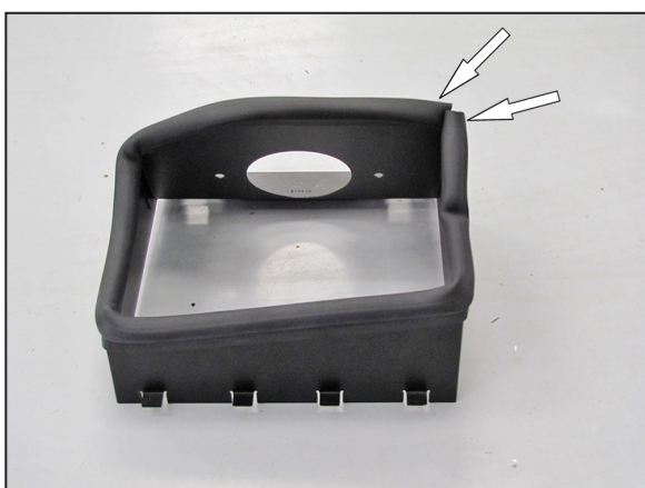
8. Install the provided edge trim onto the heat shield as shown. NOTE: Some trimming of the edge trim will be necessary.
