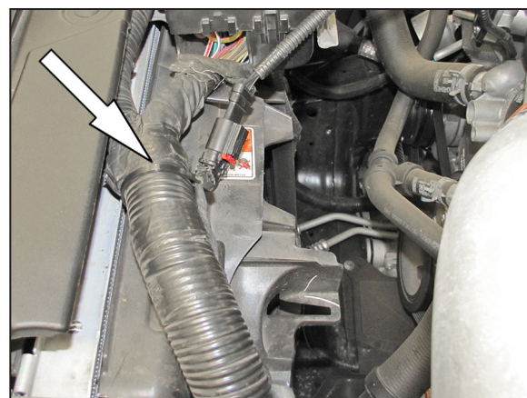
21. Secure the mass air wiring to the factory wiring harness with the provided tie wrap.
