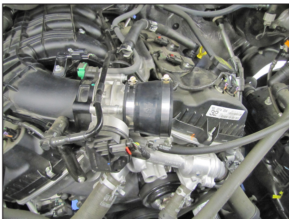
7. Install the provided silicone hose (08724) onto the throttle body and secure with the provided hose clamp.
