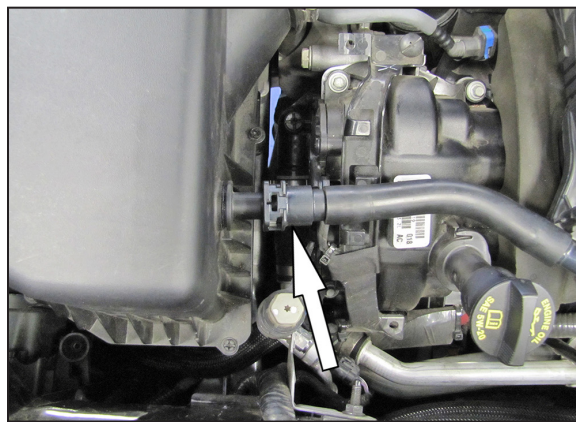
3. Disconnect the crank case vent hose from the air filter housing.
