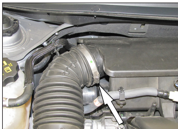
4. Loosen the hose clamp that secures the intake tube to the intake plenum.
