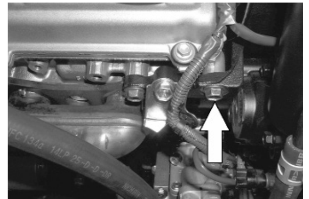
18d. On 2003 models, remove the bolt from power steering bracket as shown
