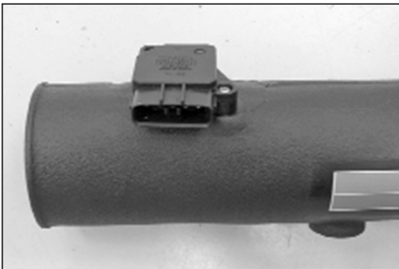
10. Install the mass air sensor into the K&N® intake tube using screws and spacers provided.
