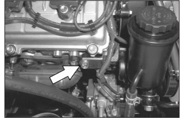
18b. On 2003 models, loosen and remove the bolt that secures the wire harness bracket located directly behind the power steering reservoir.
