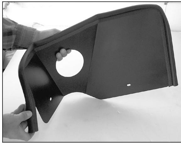
13. Install the edge trim onto the heat shield as shown above. Trim if needed.
