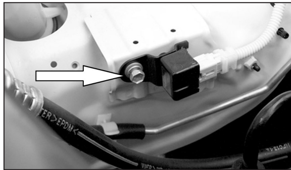
17. Remove the bolt from the relay bracket as shown.
