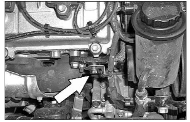
18a. On 2000-02 models, loosen and remove the bolt that secures the wire harness bracket located directly behind the power steering reservoir.
