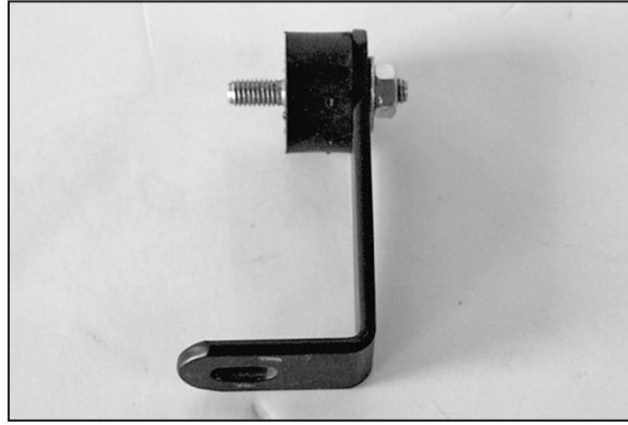
14. Assemble the "L" bracket and rubber mounted stud as shown.
