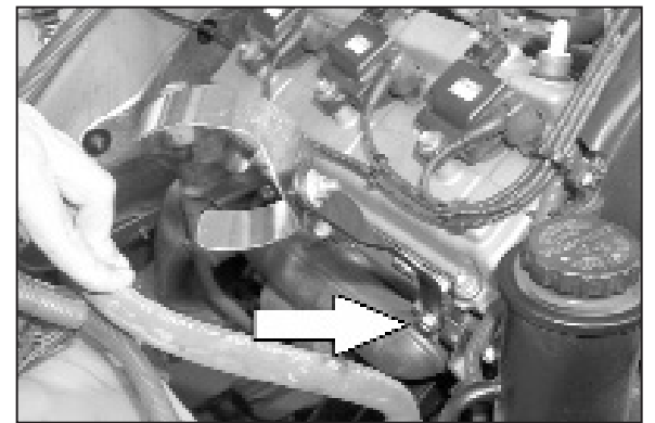
19. Install the saddle bracket assembly onto the motor using the bolt from step 18. Do not tighten completely.
