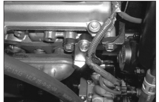
18c. On 2003 models, remove wire harness from bracket then turn bracket over and mount to engine as shown, then re-install wire harness.
