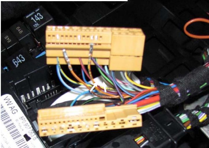
Montageposition 7 / Assembly position 7
