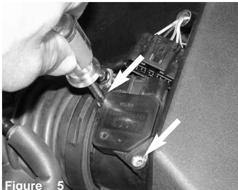
Figure 5 With Phillips screwdriver, loosen the 2 screws that secure the MAF sensor to the sensor housing.
