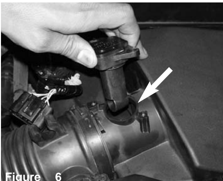
Figure 6 Carefully, remove MAF sensor from the air box sensor housing.
