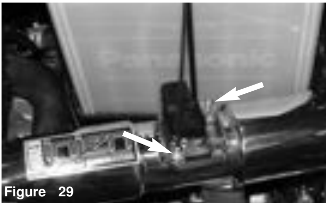
Figure 29 The two m4 x 10mm bolts in this kit are used to fasten the mass air flow sensor in place.
