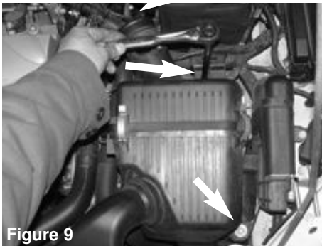
Figure 9 Use a 10mm socket, extension and ratchet and loosen the two 10mm bolts on the air box assembly.
