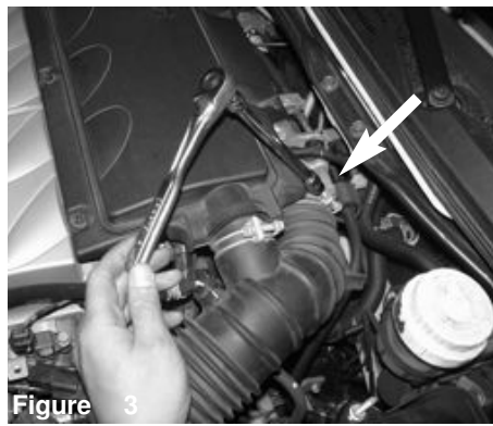
Figure 3 Loosen the clamp on the intake air duct attached to the throttle body
