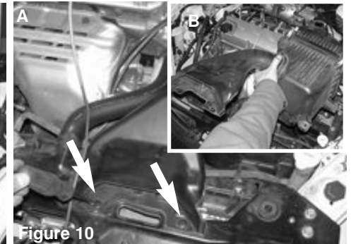
Figure 10 Figure A: Remove the two plastic screws on the air box scoop. Figure B: Remove the entire air box assembly
