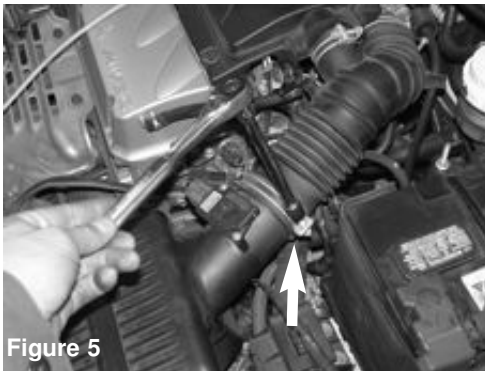
Figure 5 Loosen the clamp on the air duct attached to the air box assembly.
