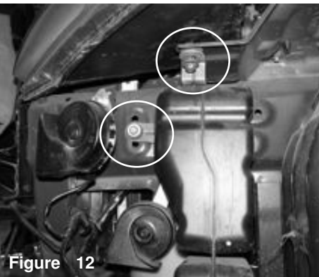
Figure 12 You will now need to remove the front bumper. Looking at the driver side corner, you'll notice the remaining two m6 bolts that will be removed from the air box resonator brackets. These bolts will need to be removed
