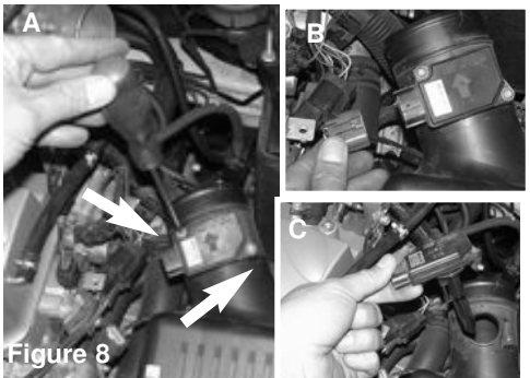
Figure 8 Figure A: Use a torx screw driver to remove the two torx screw attached to the MAF sensor. Figure B: Unplug the MAF sensor harness. Figure C: Remove the MAF sensor from the air box assembly
