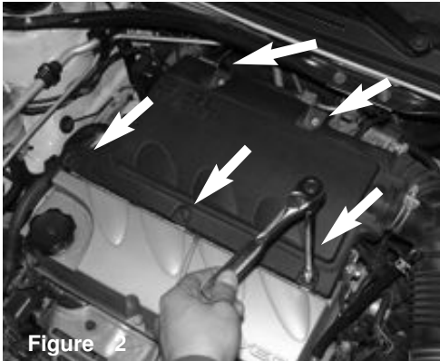
Figure 2 Use a 10mm Socket and ratchet and remove the 5- 10mm bolts on the intake resonator located on top of the valve cover
